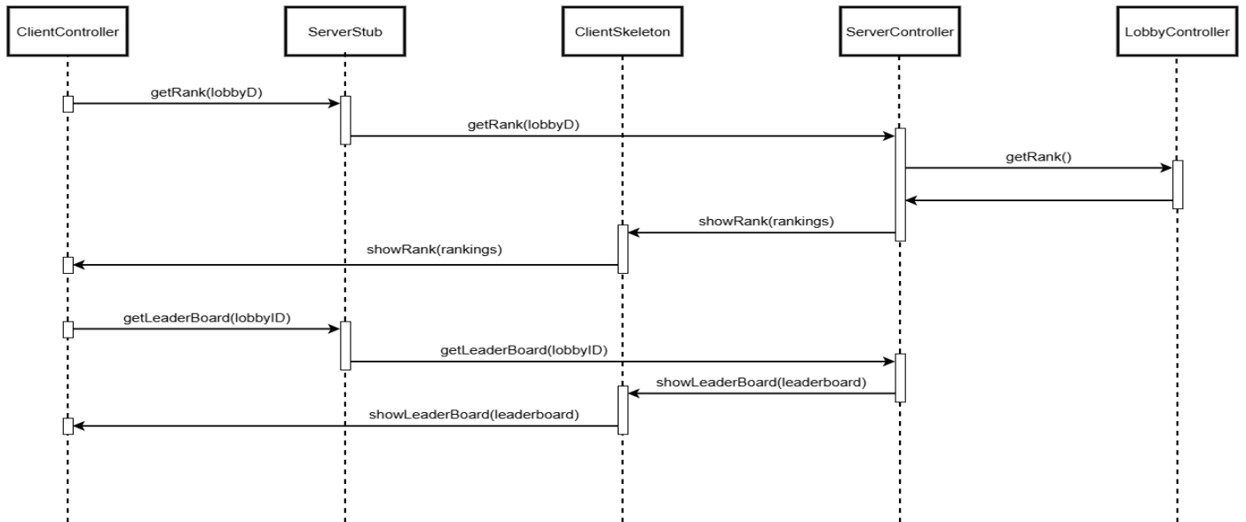
Rank RMI Sequence Diagram
