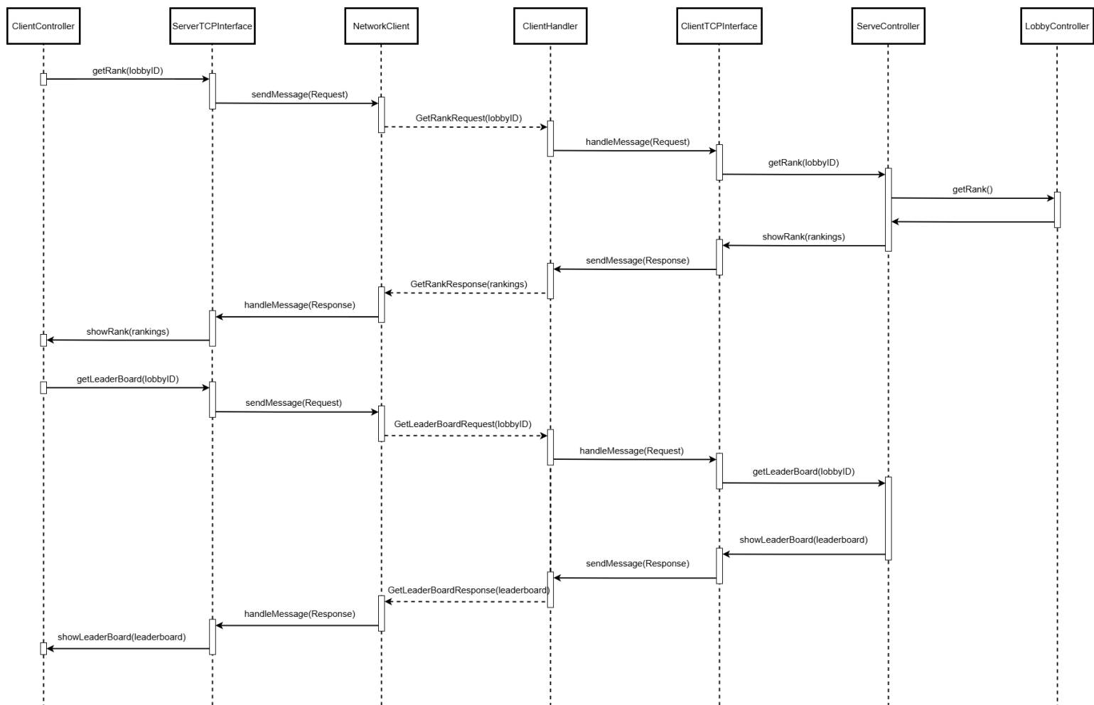
Rank TCP sequence diagram
